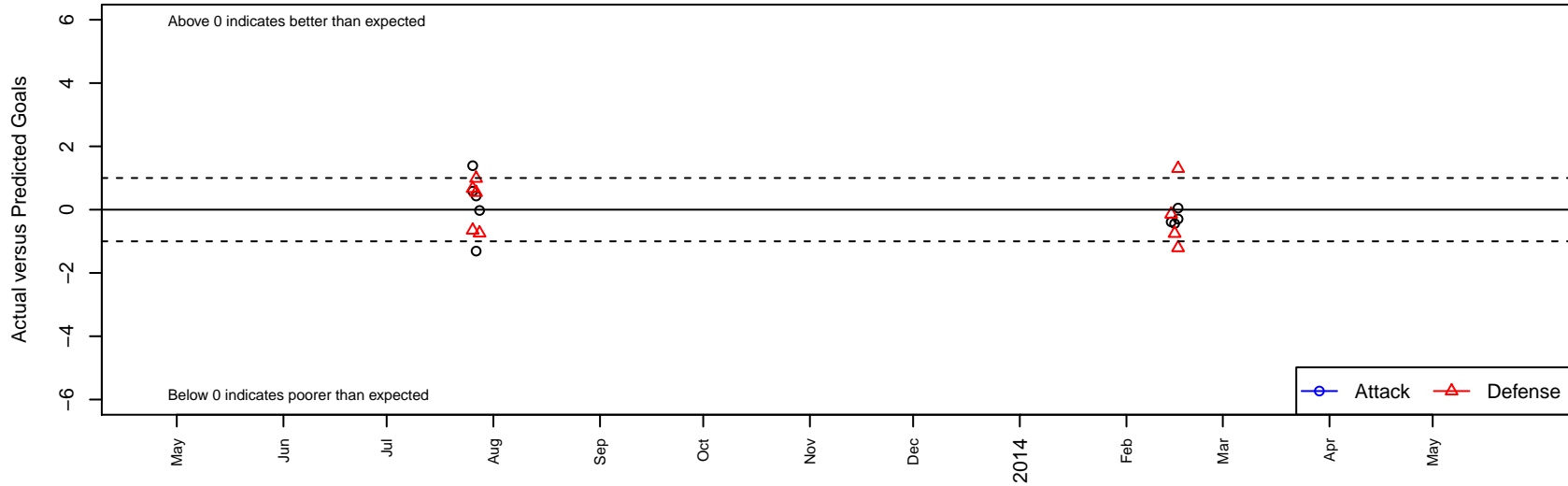
Alaska Rush 02 G01 Dots are actual minus expected GF (blue circles) and GA (red triangles). Blue line is smoothed change in attack strength. Red is smoothed change in defense strength.
